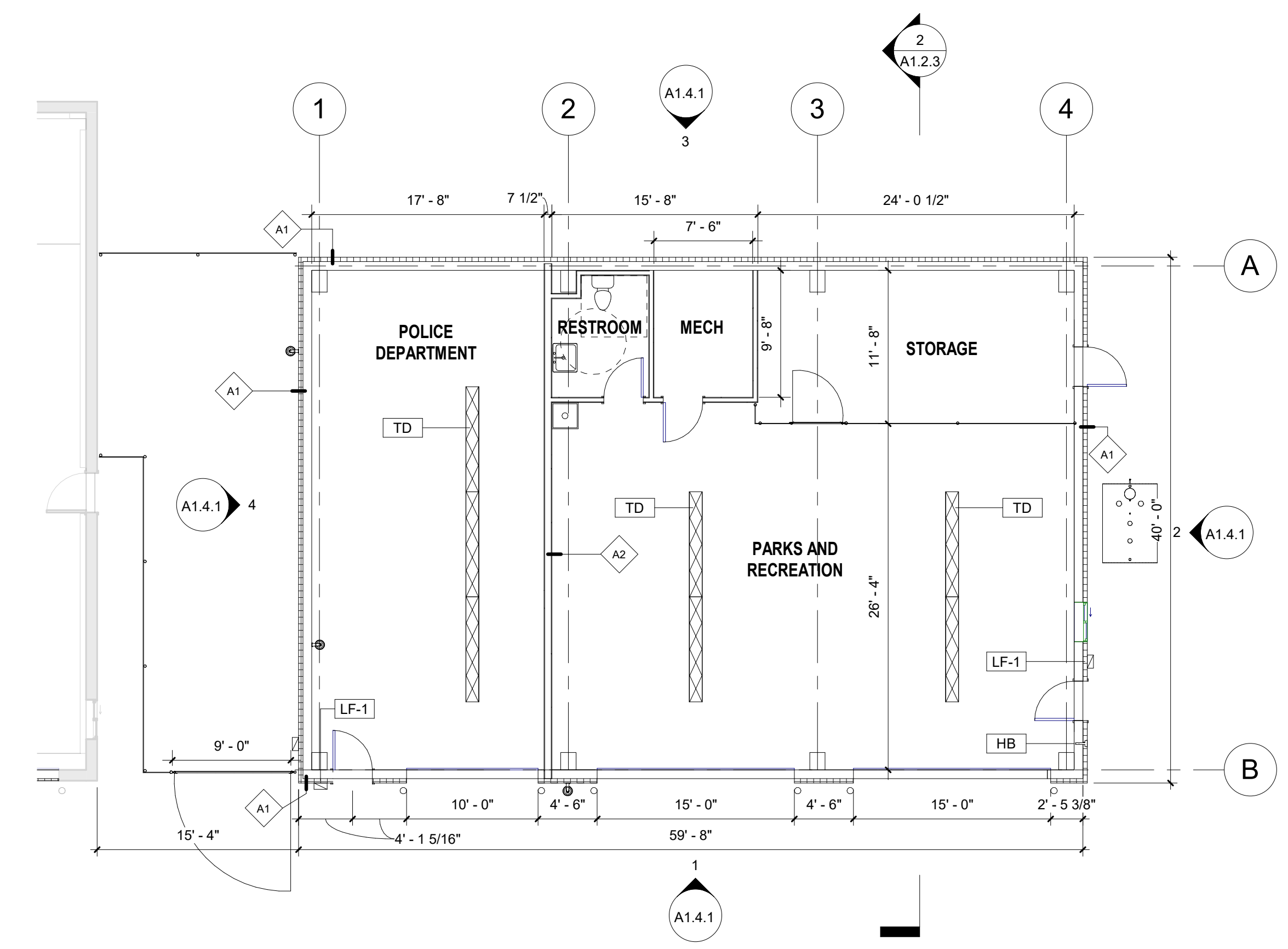
1 CONDITIONED POLE BARN FLOOR PLAN 1/8" = 1'-0"
