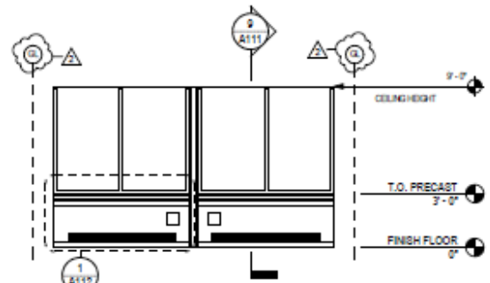
2 INT. ELEV. - CLASSROOM - EXISTING A111 1/4" = 1'-0"
