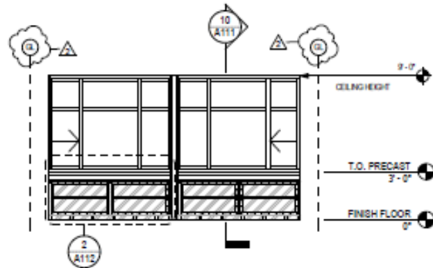
4 INT. ELEV. - CLASSROOM - NEW A111 1/4" = 1'-0"
