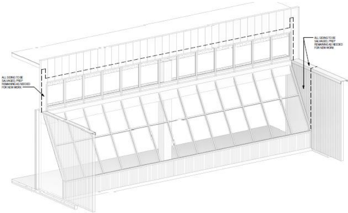
1 A113 AXON - CAFETERIA WINDOW - EXISTING
