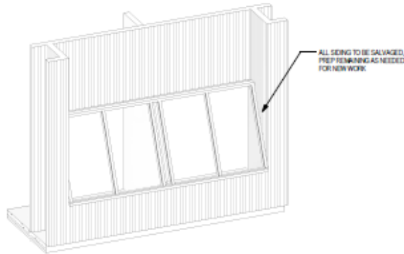
1 CLASSROOM WINDOW - EXISTING A111
