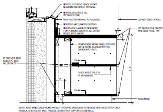
3 CLASSROOM COUNTERTOP - NEW A112 1 1/2" = 1'-0"
