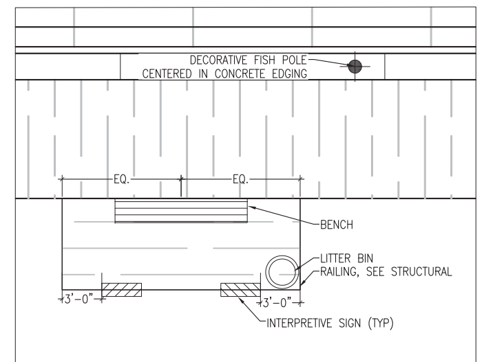
BENCH OVERLOOK LAYOUT (TYP)
