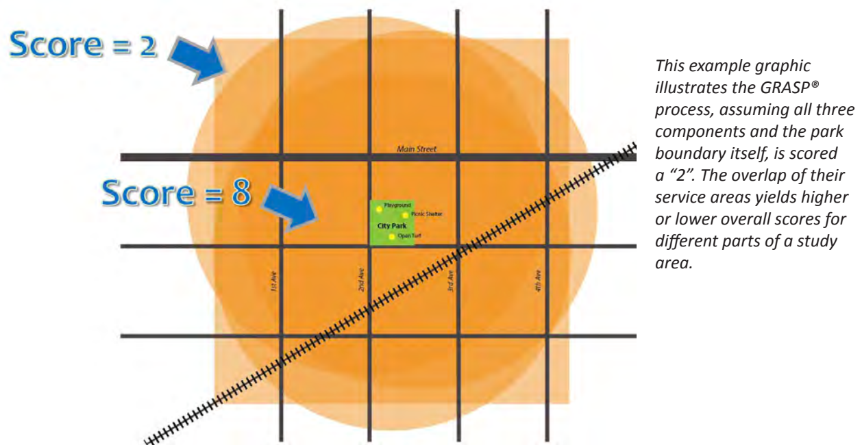
Figure 47: GRASP® Process
