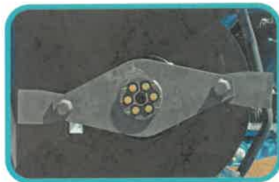
Two double-sided blades on a 5/8" thick blade carrier
